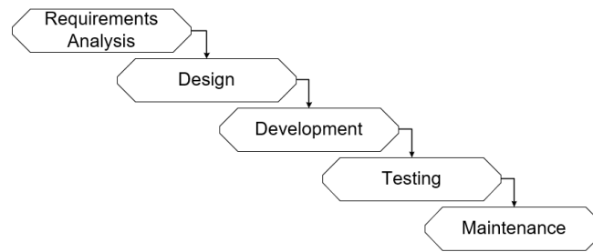
Gambar 1. Metode Waterfall
